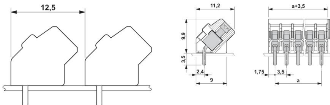
Dimensioned drawing
